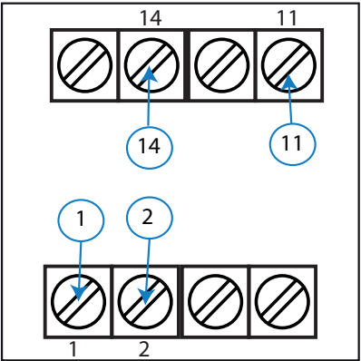
Figura 3:Bornes DCB-48 Vac.
