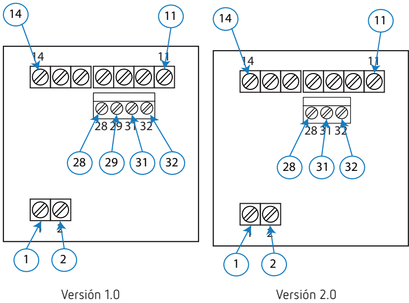
Figura 3:Bornes DCB-72 Vac.
