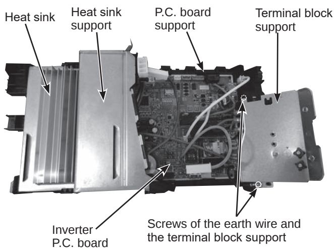
Photo 5 (Inverter assembly)
