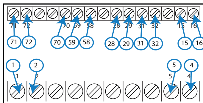
Figura 3: Bornes DHC-96 Aac.
