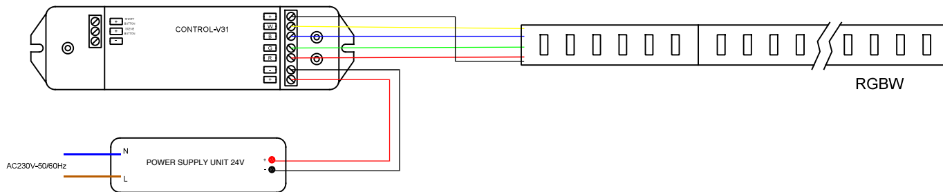
Figure 1. Connection scheme.
