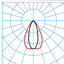
Mirona Fit T LED26000-840 TX050472
