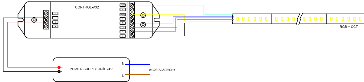
Figure 1. Connection scheme.
