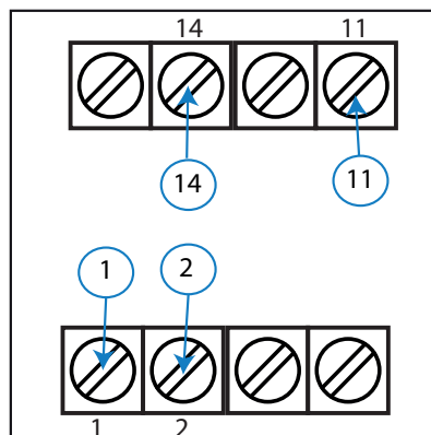
Figura 3: Bornes DCB-48 Vdc.
