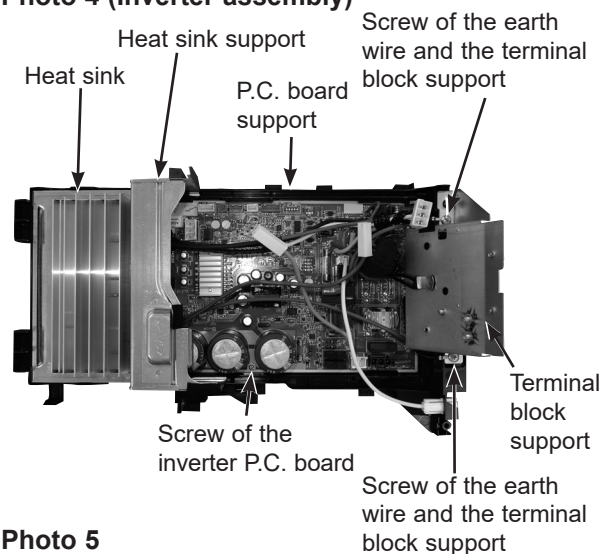
Photo 4 (Inverter assembly)
