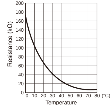
Fin temperature thermistor (RT64)
