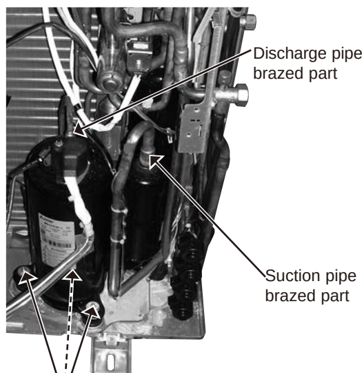
Compressor nuts
