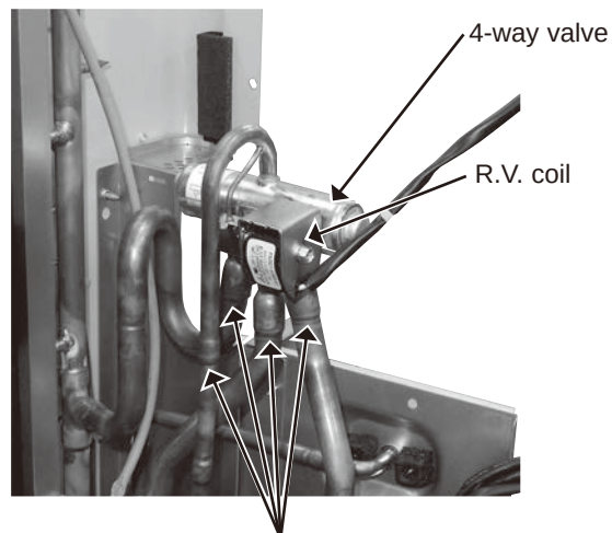
Brazed parts of 4-way valve and pipes
