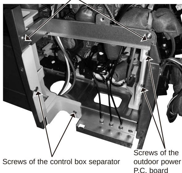
Screws of the TB support
