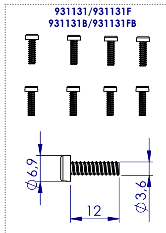
Ref. T-1316/1 TORNILLOS (8) SCREWS VIS
