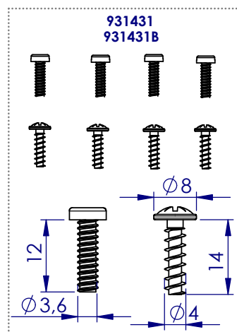
Ref. T-1316/1 TORNILLOS (4) Ref. T-1316/2 TORNILLOS (4) SCREWS VIS
