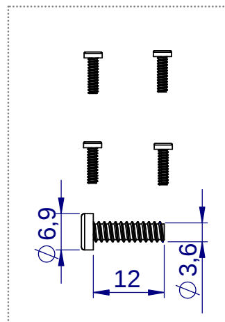
Ref. T-1316/1 TORNILLOS (4) SCREWS VIS
