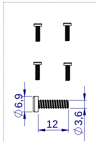
Ref. T-1316/1 TORNILLOS (4) SCREWS VIS
