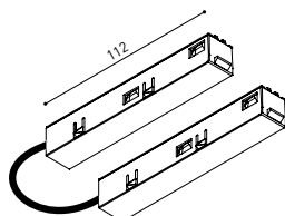
TRACK 48V Corner Connector
