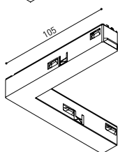
TRACK 48V Corner 90° Connector One Plane
