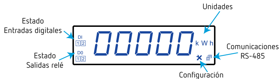
Figura 6: Display CVM-D41 DC.
