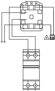
ELB(MCCB) & Relay contactor
