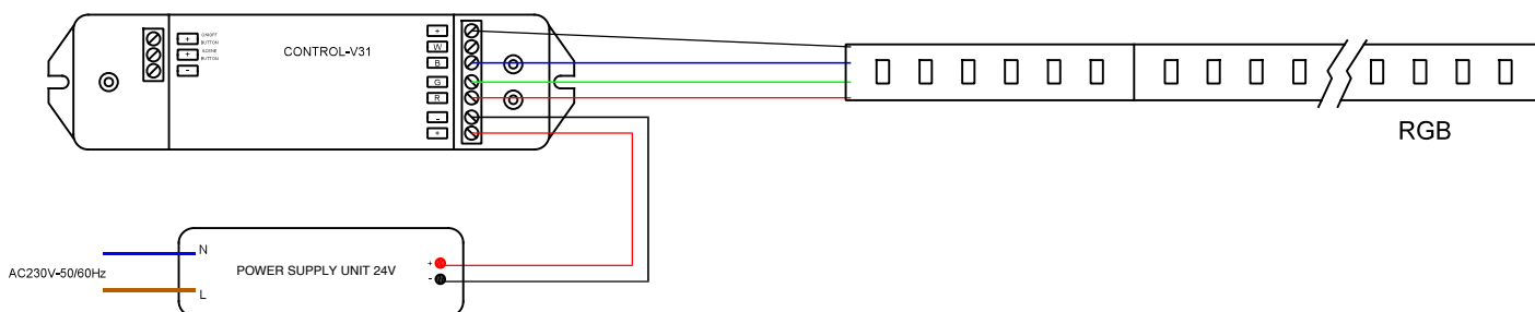
Figure 1. Connection scheme.
