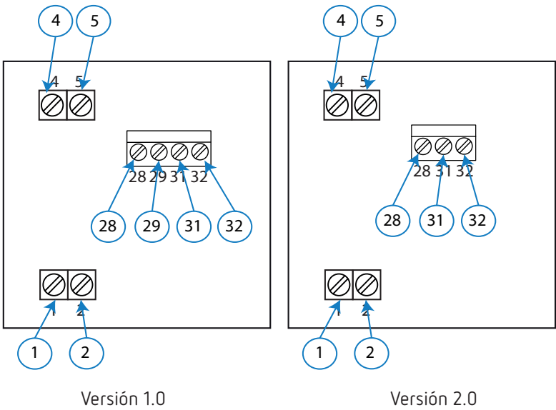
Figura 3:Bornes DCB-72 Adc.
