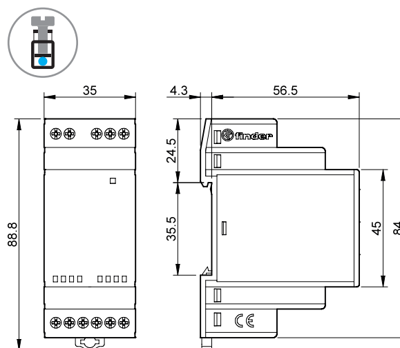
Type 70.51.0.240.N032 Screw terminal
