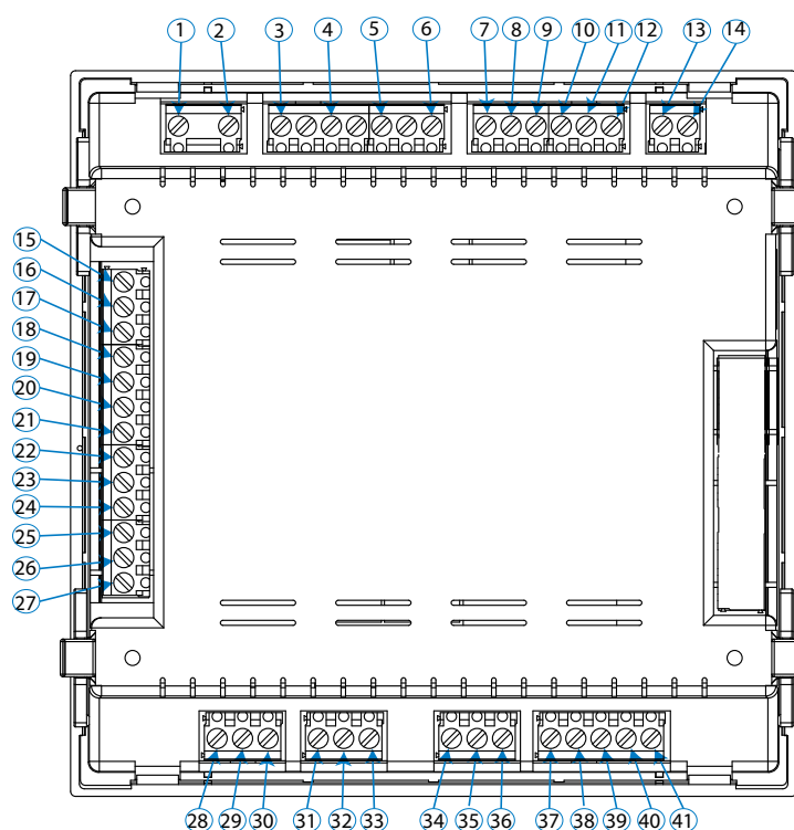
Figura 2: Bornes Computer SMART III FAST 12Vdc.
