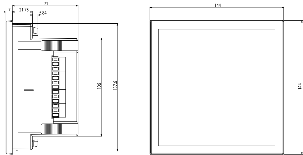
Figura 18: Dimensiones del Computer SMART III FAST. 12Vdc
