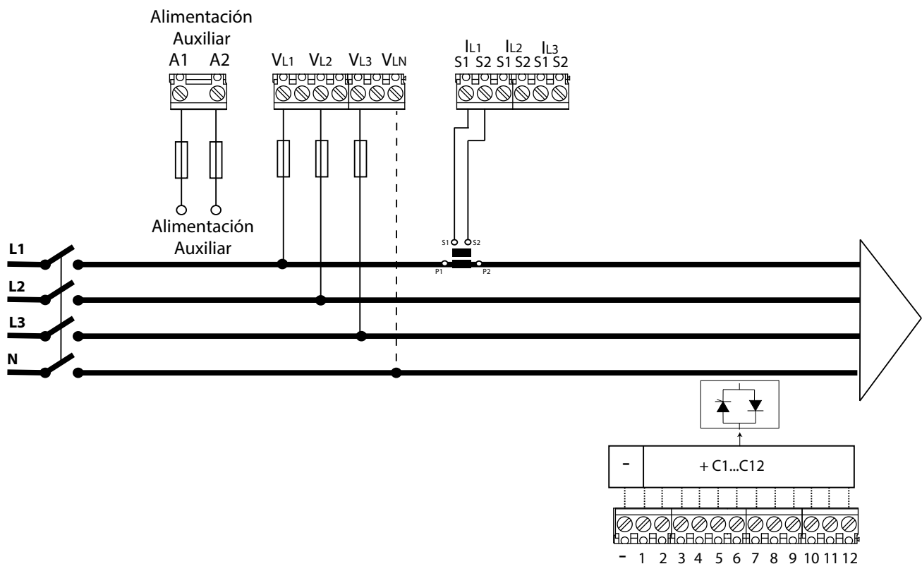
Figura 6: 3 tensiones + neutro y 1 corriente, modelo Computer SMART III 12 FAST 12Vdc.
