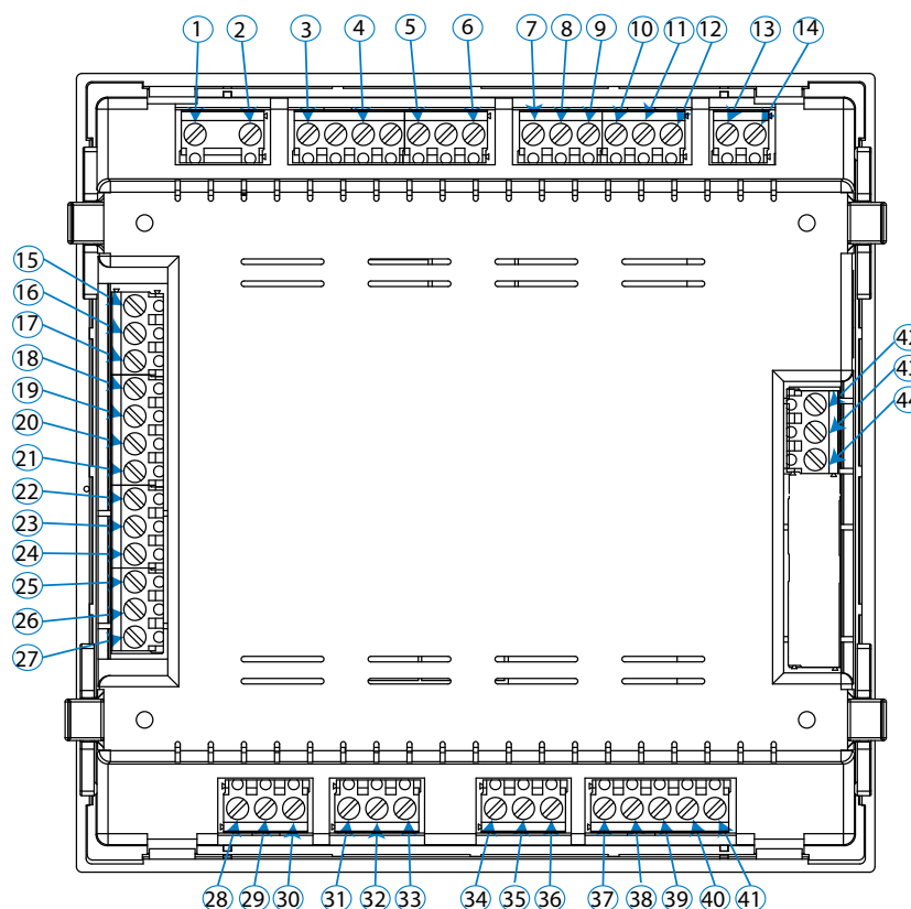
Figura 2: Bornes Computer SMART III.
