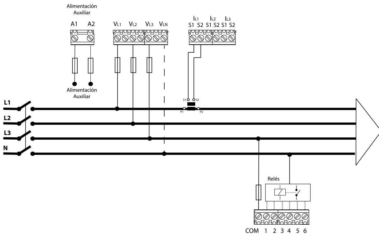
Figura 6: 3 tensiones + neutro y 1 corriente, modelo Computer SMART III 6.
