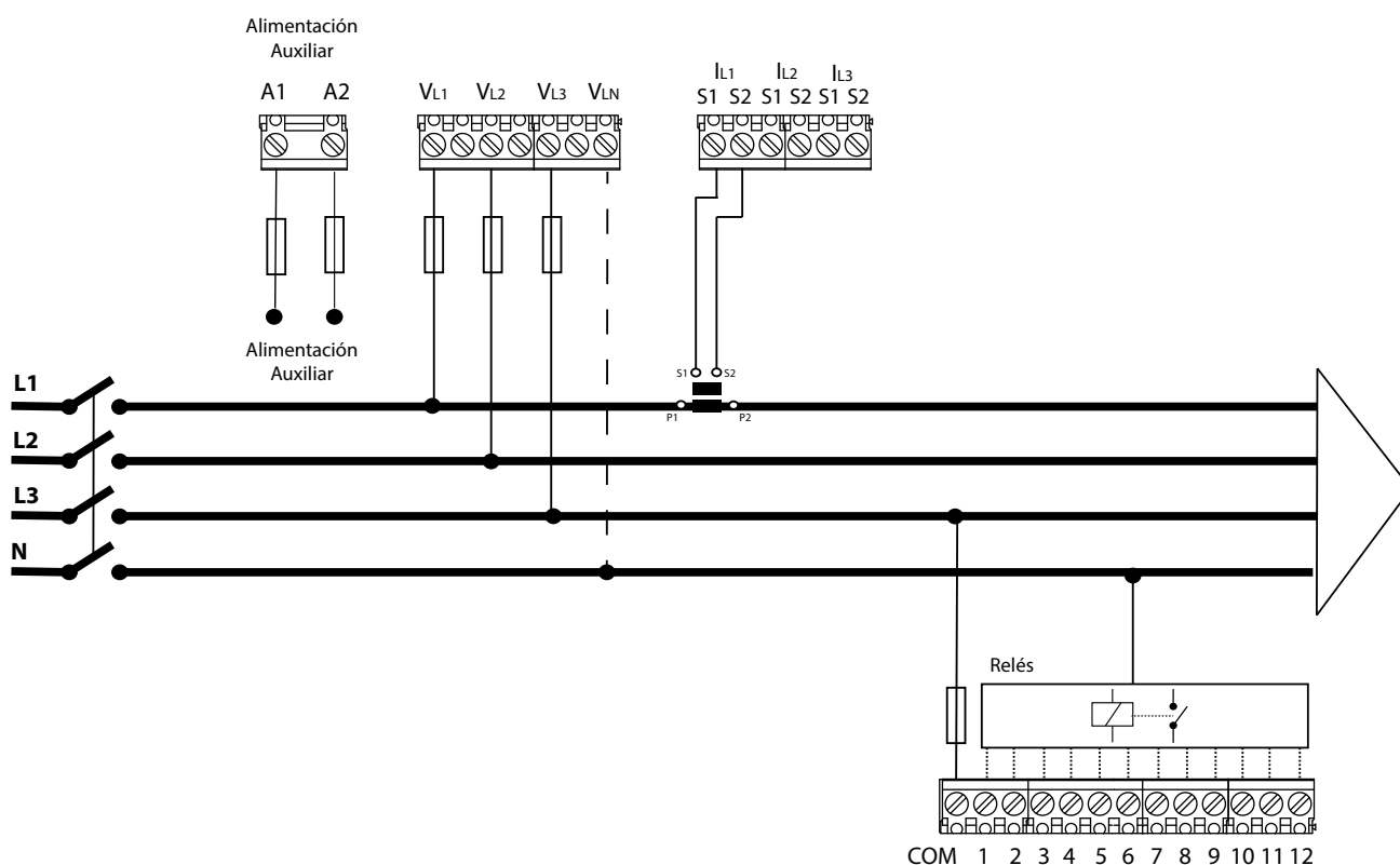
Figura 7: 3 tensiones + neutro y 1 corriente, modelo Computer SMART III 12.
