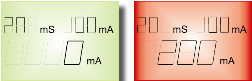
Figura 9: Display RGU-10B.
