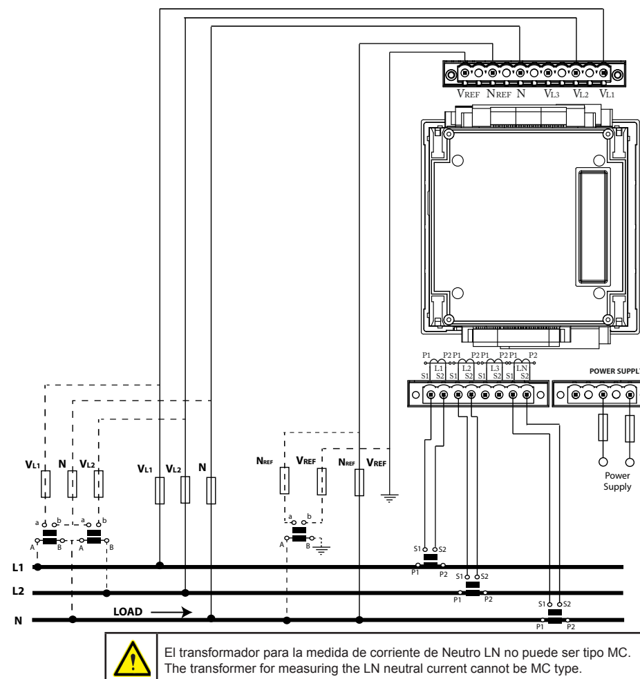
Red bifásica a 3 hilos / 3-wire two-phase network Transformadores de corriente .../5A, .../1A o .../0.250A (MC1) .../5, .../1A or .../0.250A (MC1) current transformers
