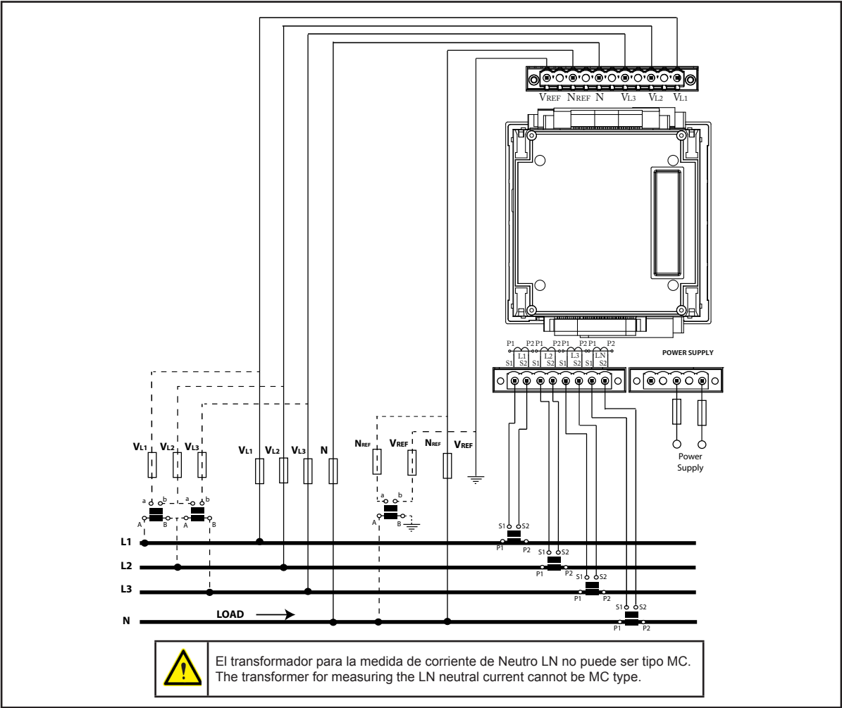
Red trifásica a 4 hilos / 4-wire three-phase network Transformadores de corriente .../5A o .../1A / .../5 or .../1A current transformers
