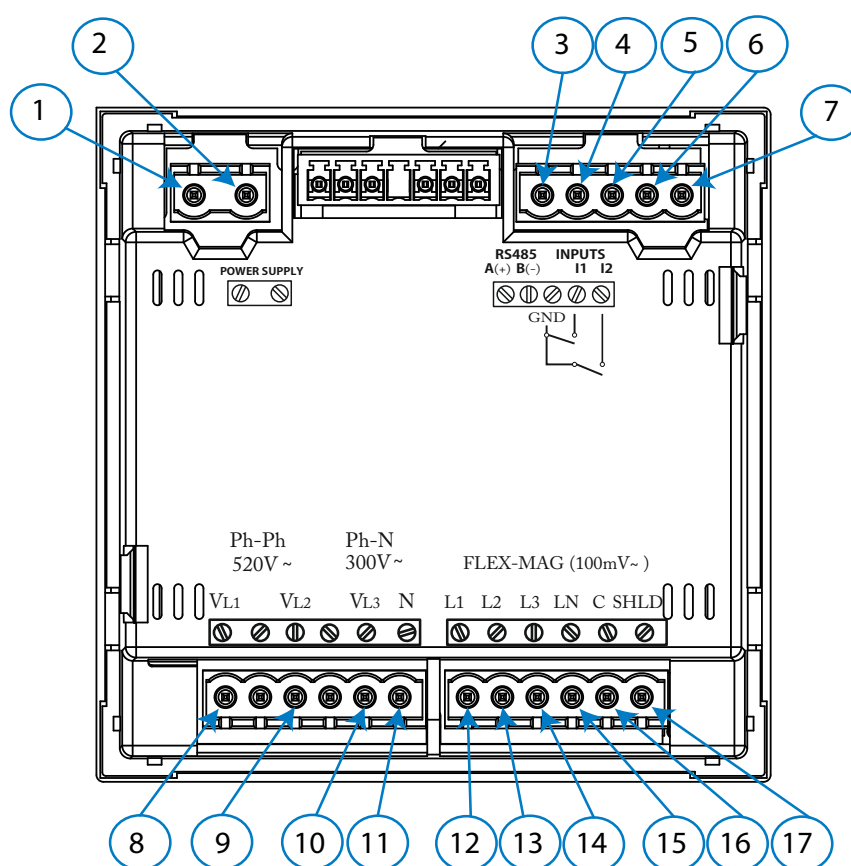
Figura 3: Bornes del CVM-C10-FLEX.
