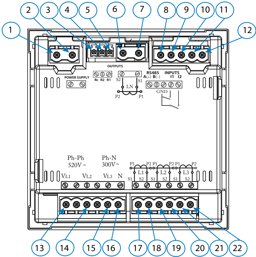
Figura 2: Bornes del CVM-C10-ITF-IN y CVM-C10-MC-IN.
