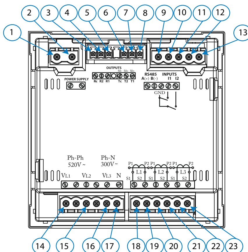
Figura 1: Bornes del CVM-C10-ITF, CVM-C10-MC y CVM-C10-mV.
